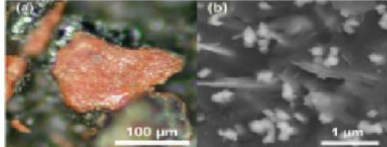
Highly energetic rod-like chip discovered in the WTC dust at optical magnification (a) and 50,000x electron microscope magnification (b). The latter image shows consistently sized iron oxide particles approximately 100 nm across and 40 nm-thick walls of aluminum embedded in carbon-rich matrix.
